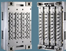
Pet Preform Mould 32 Cavity
